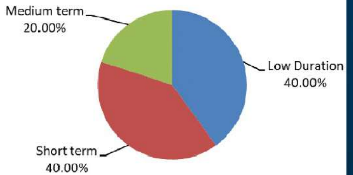
Category exposure
