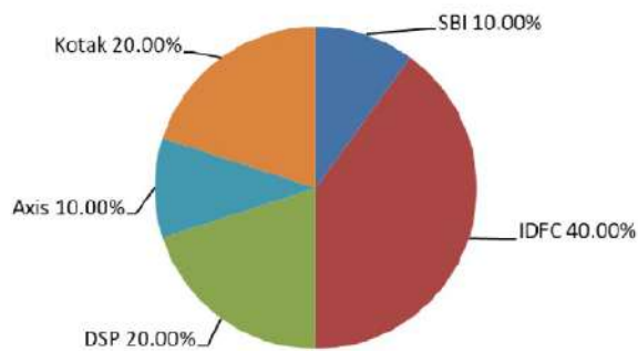
AMC exposure
